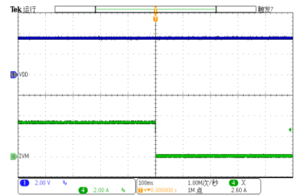
Increase I_{VM} to OCP Point
