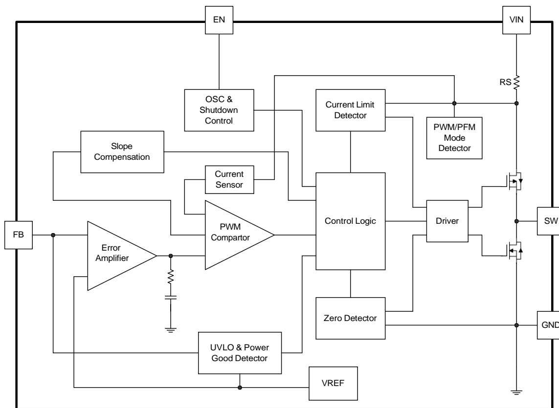
RP3420SOT5 Block Diagram
