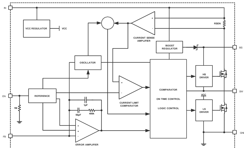
RP8326SO8 Block Diagram
