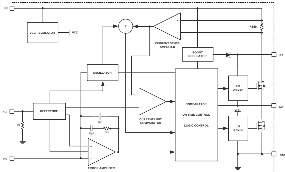
Figure 2. RP3834ES8 Block Diagram
