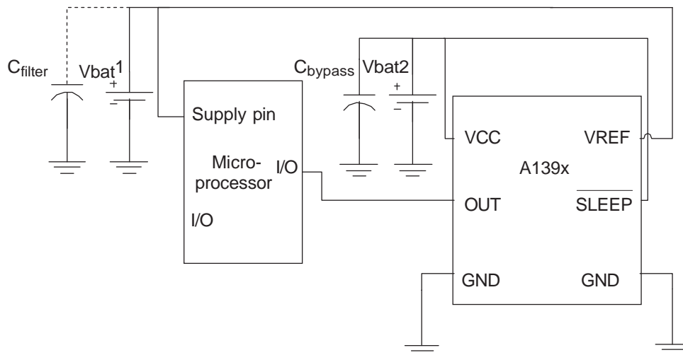
Figure 4. Application circuit showing ratiometry of V_{REF} . Sleep mode is disabled and the VREF pin is tied to the microprocessor supply.
